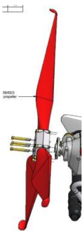
R108752 HELICE ARPLAST 158/62/3 (Curved Tip)
