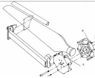
R108770 HELICE ARPLAST 166/48/4
